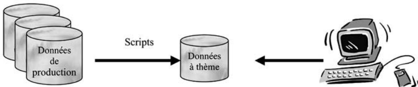
Figure 51. Architecture Datamart
