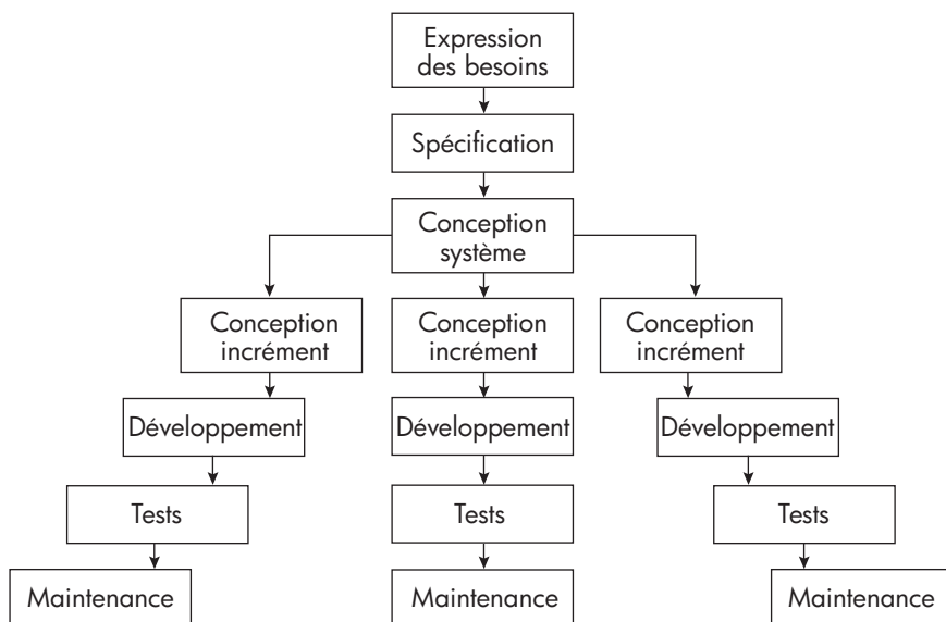
Figure 16. Cycle incrémental
