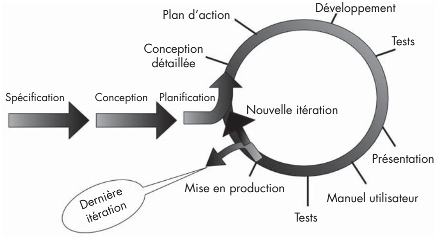
Figure 25. Cycle Crystal
