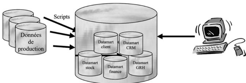
Figure 52. Architecture Datawarehouse
