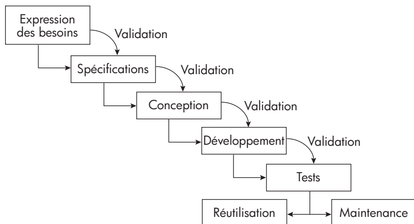
Figure 15. Cycle RAD
