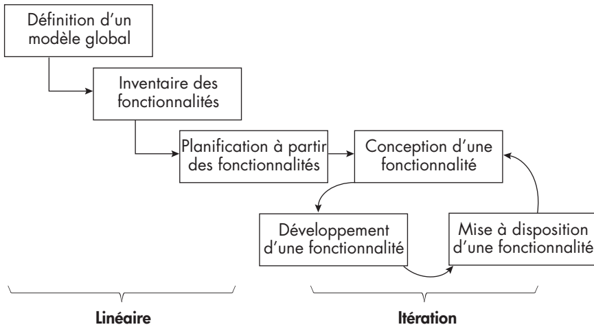
Figure 24. Cycle FDD
