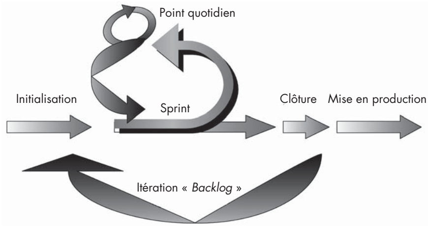
Figure 26. Cycle SCRUM
