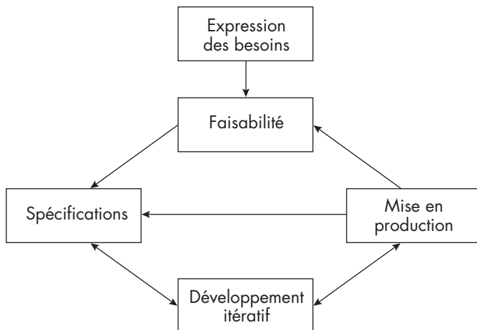
Figure 23. Cycle DSDM
