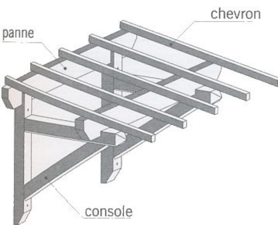
fig. 5.34 auvent
