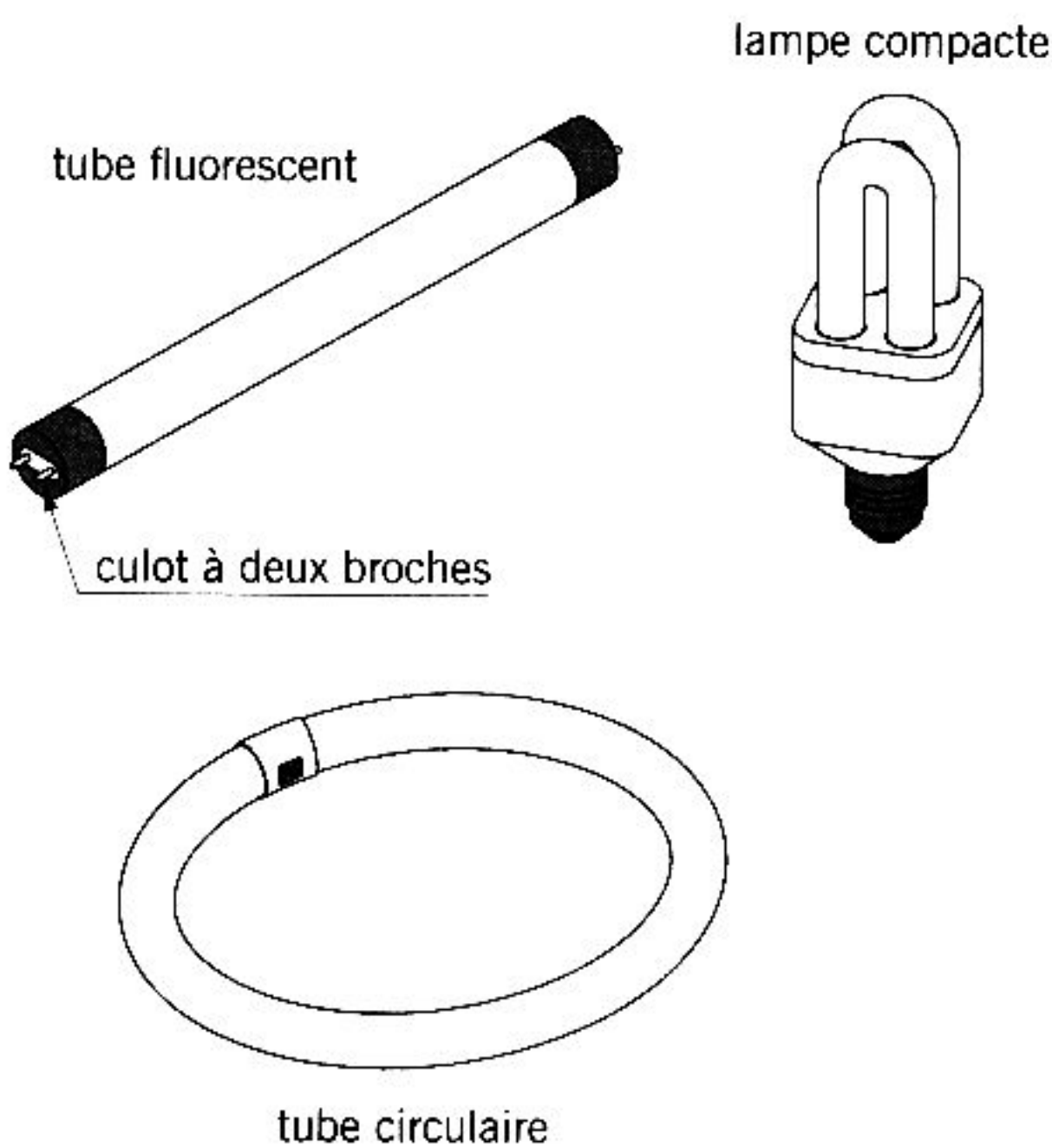
fig. 16.33 tubes fluorescents
