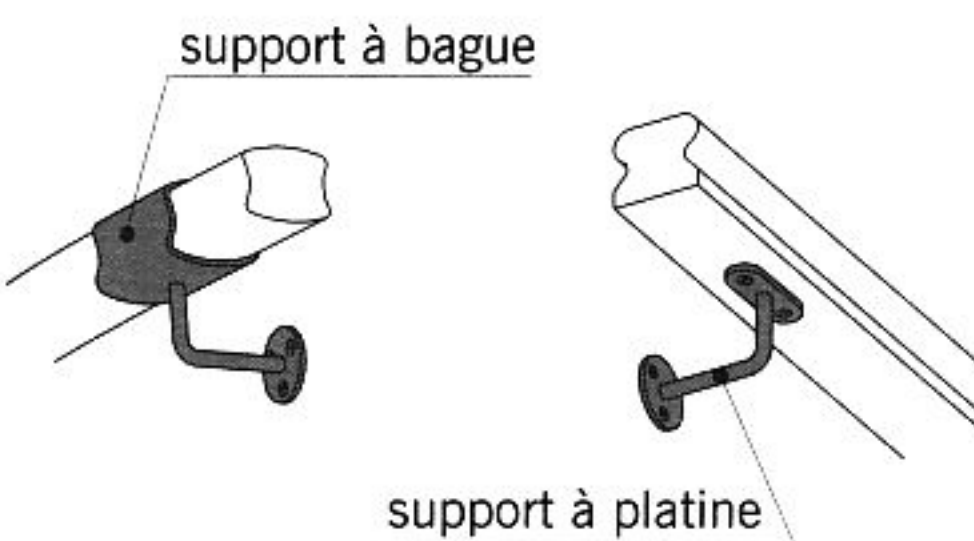
fig. 13.44 supports
