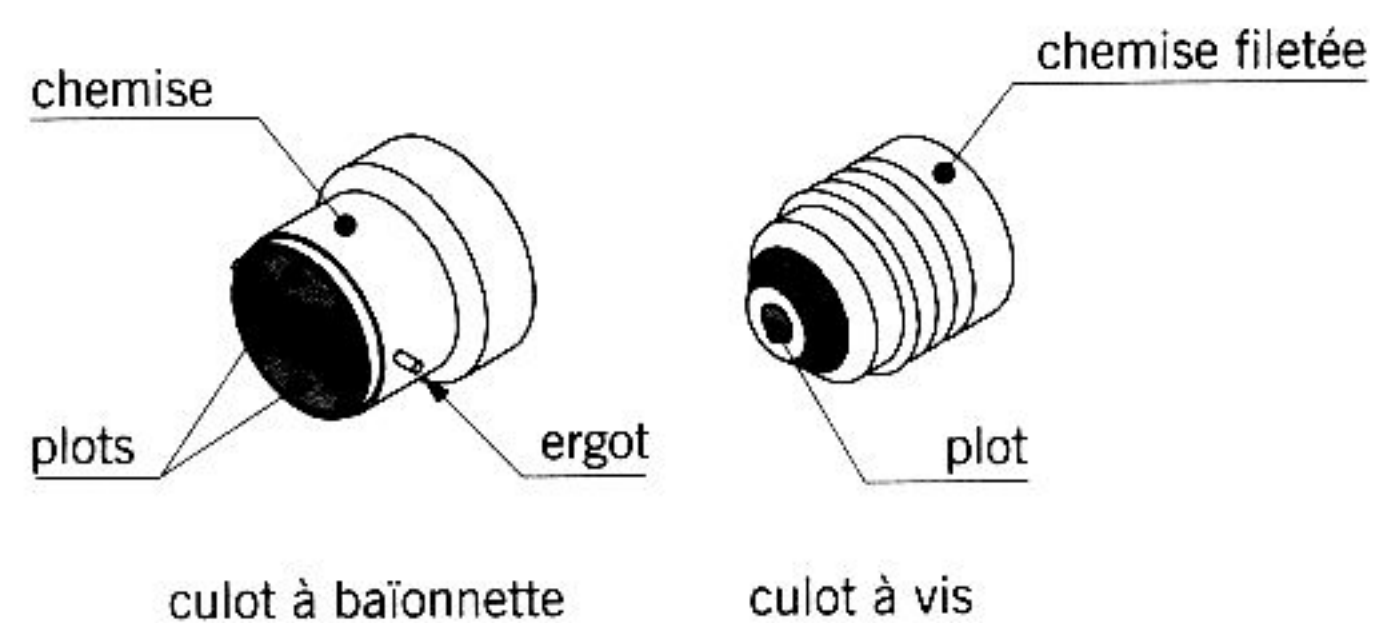
fig. 16.31 culots
