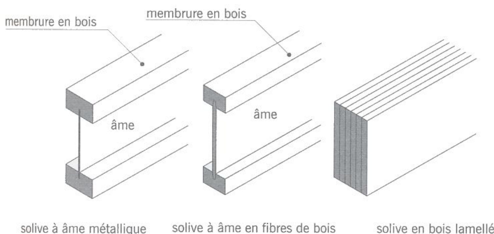
fig. 4.22 solives composites
