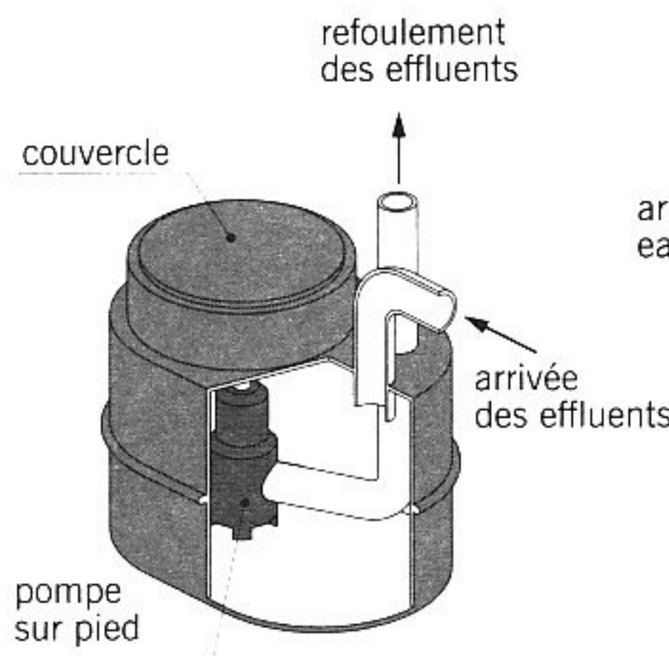
fig. 15.12 mini-station
